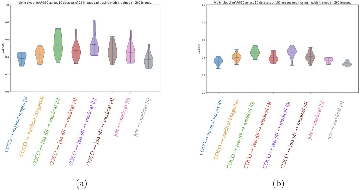
Figure 6.8: Comparison of the two violin plots for the models trained on 200 images, one for test sets of 25 images each (a) and one for test sets of 100 images each (b)
