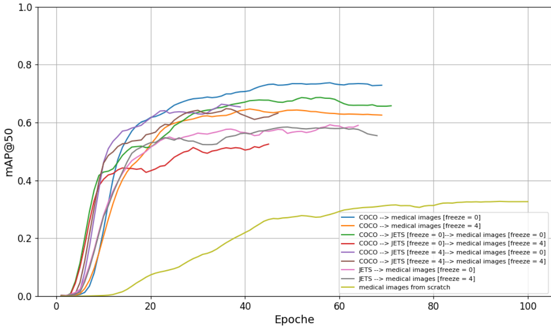
Figure 6.5: mAP@50 evaluated on the validation set after each training epoch. The different lines represent the models trained with different pre trained weights and different number of frozen layers.
