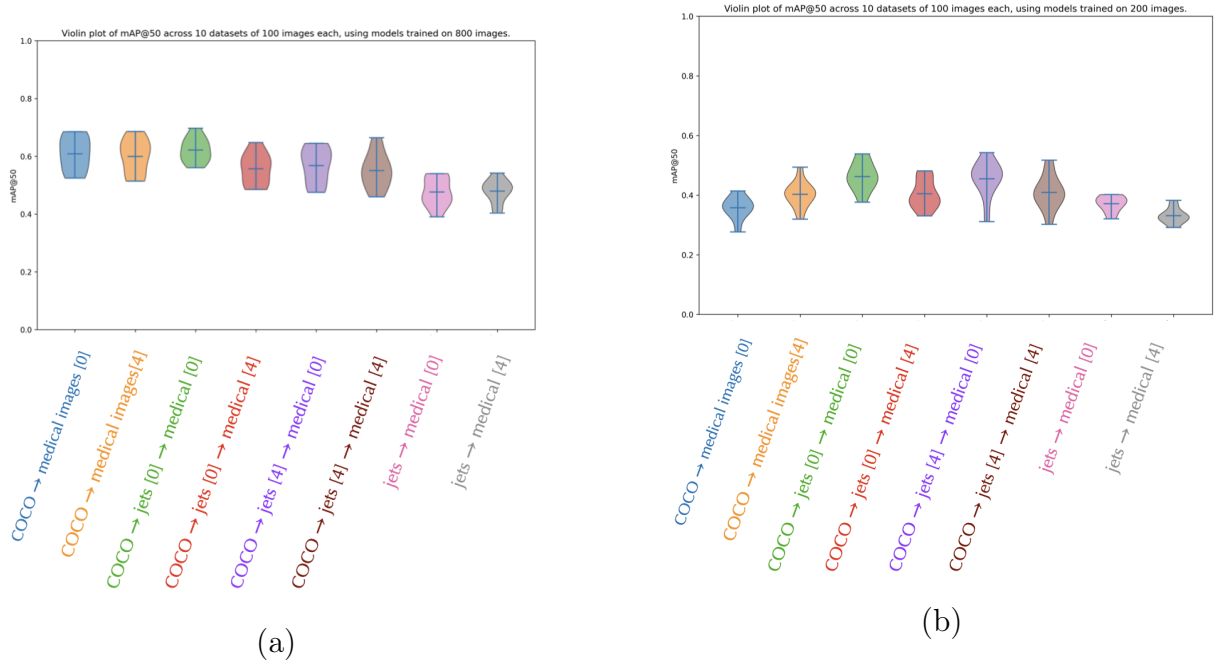
Figure 6.9: Distribution of the results for the models trained on 800 images (a) and 200 images (b), both evaluated on test sets of 100 images each.
