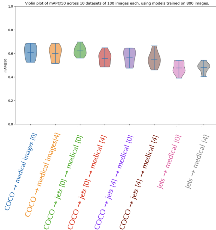
Figure 6.6: Violin plot of the mAP@50 results on the 10 different test sets for each model after training on 800 medical images. The width of each violin represents the distribution of the scores, with wider sections indicating a higher density of scores in that range. The horizontal line inside each violin indicates the mean score for that model.
