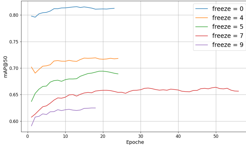
Figure 6.4: mAP@50 evaluated on the validations set after each training epoch of the last step. The different lines represent the models trained with different number of frozen layers.
