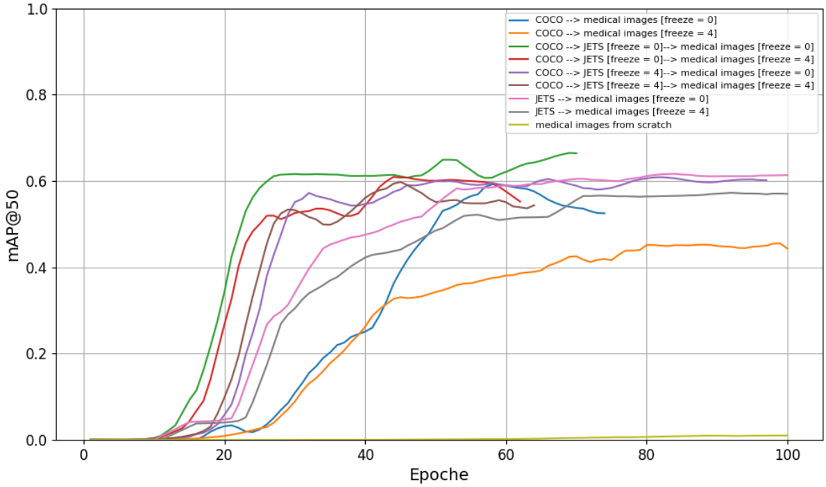
Figure 6.7: mAP@50 evaluated on the validation set after each training epoch.
