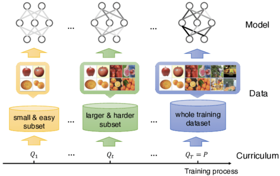
Figure 2.9: Illustration of the curriculum learning concept [15].
