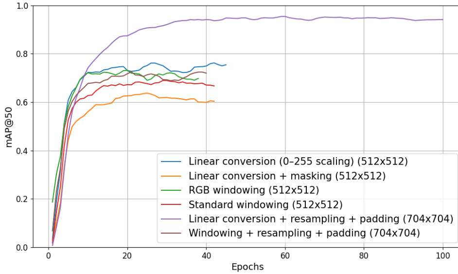
Figure 6.1: mAP@50 evaluated on the validation set after each training epoch for the different types of preprocessing.
