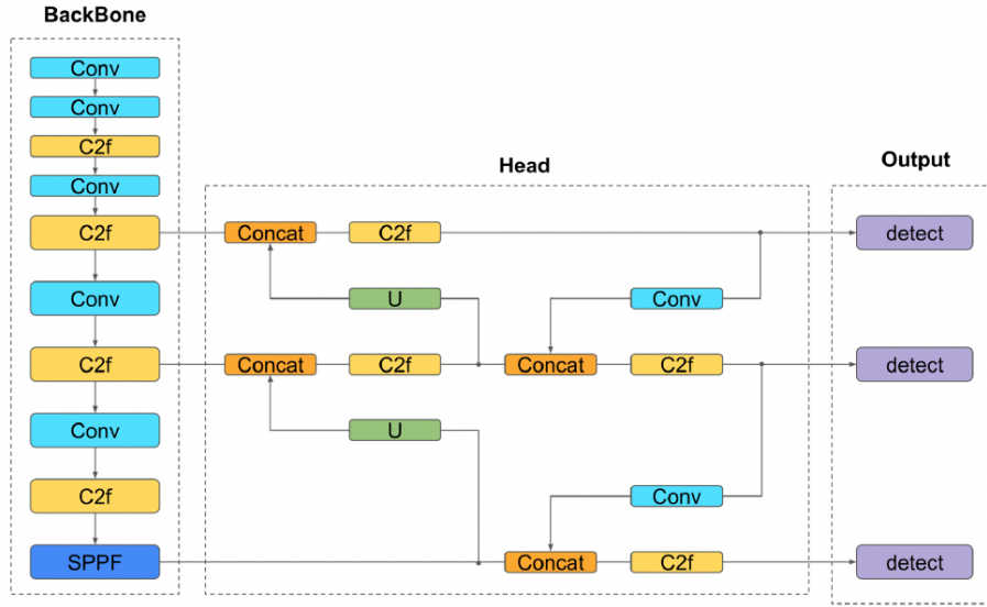
Figure 6.3: YOLOv8 architecture
