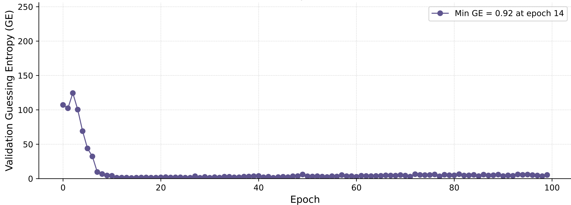
Validation GE over Epochs (Mamba Model)
