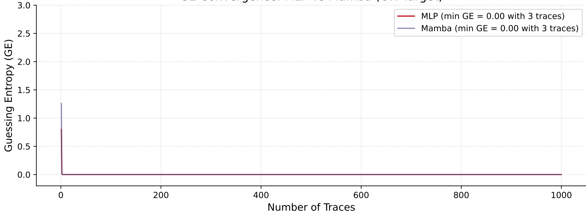
GE Convergence: MLP vs Mamba (CW-Target)
