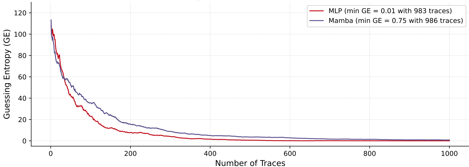
GE Convergence: MLP vs Mamba (ASCADv1)
