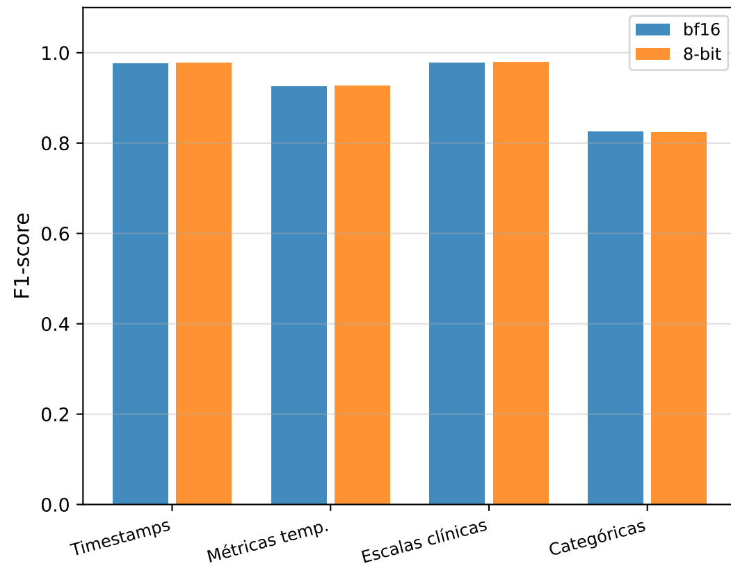
Qwen2.5-7B
