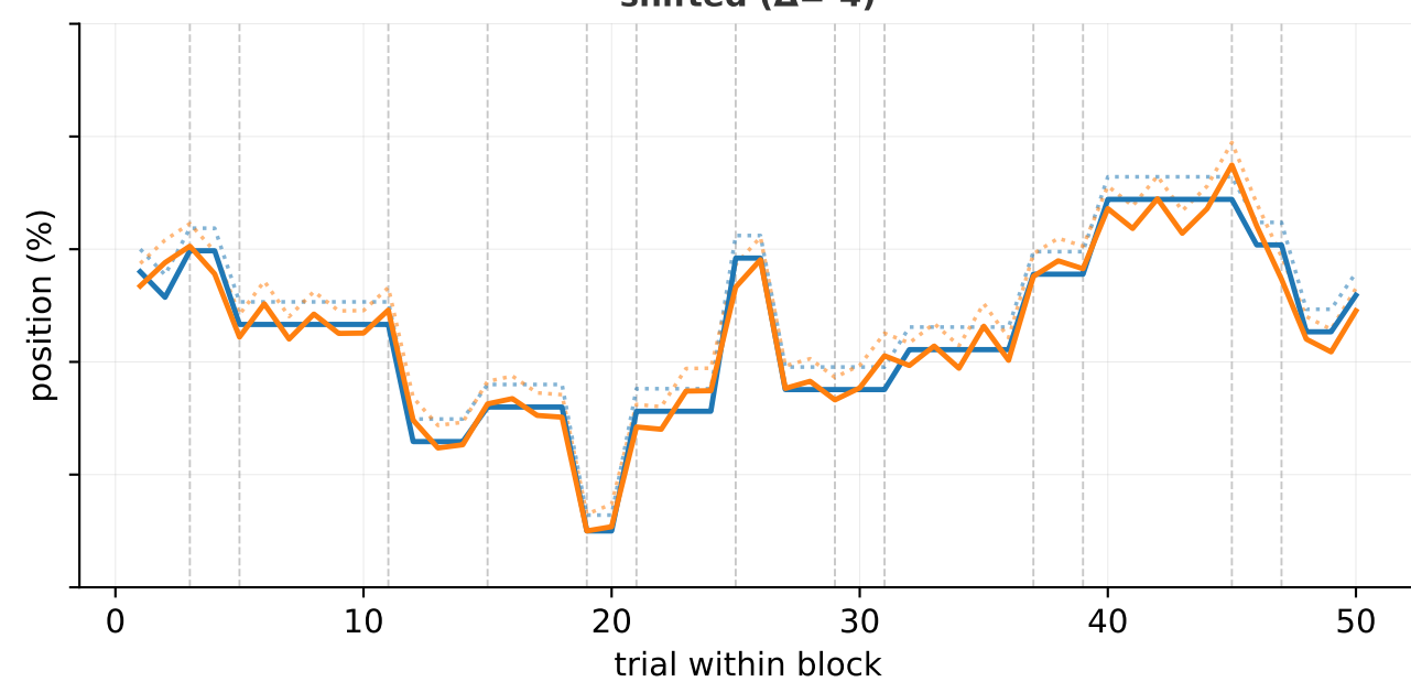
design idx 3 · vol=low, stc=high, valence=loss shifted ( \Delta=-4 )
