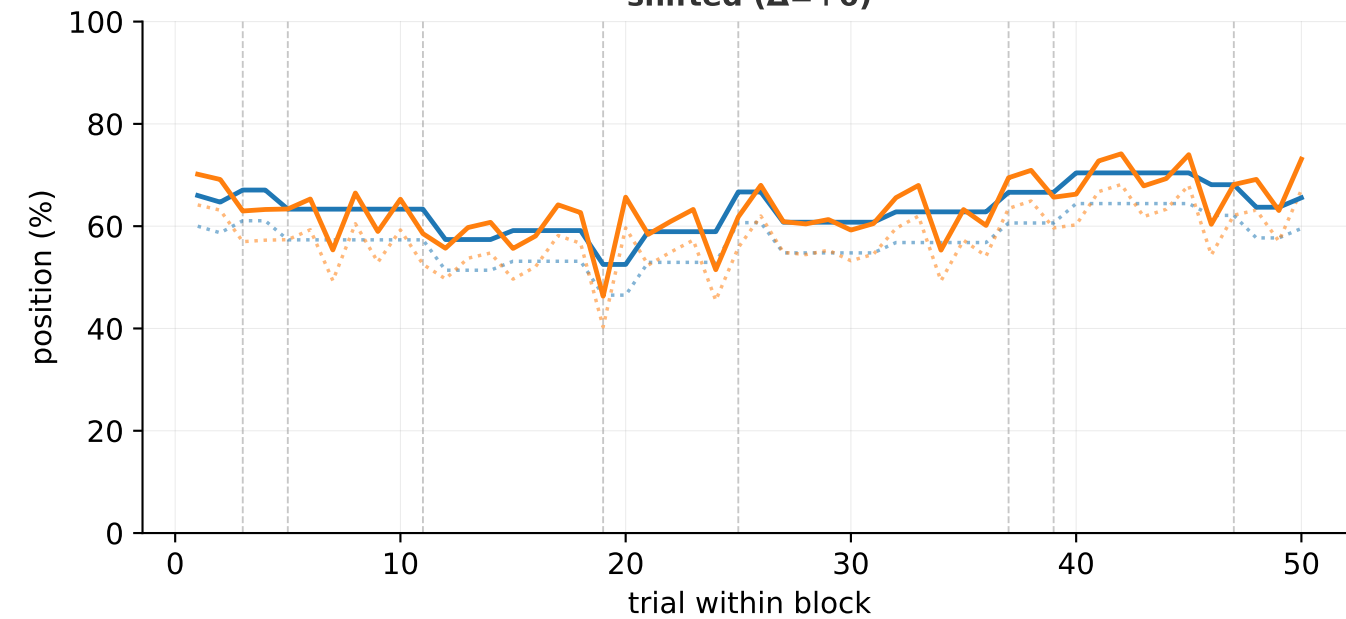
design idx 2 · vol=high, stc=low, valence=loss shifted ( \Delta=+6 )
