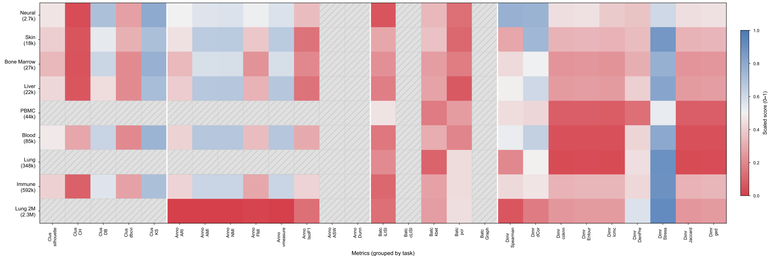
CheckAtlas benchmarking overview — scaled metric scores per atlas
