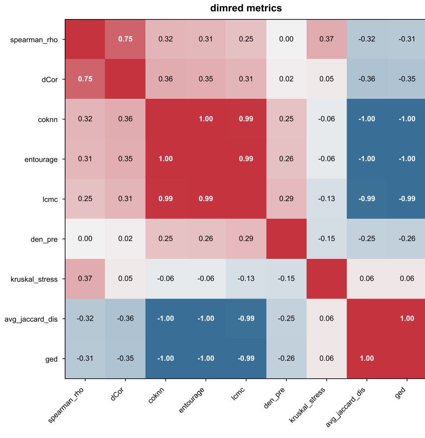
Inter-metric correlations within each task
