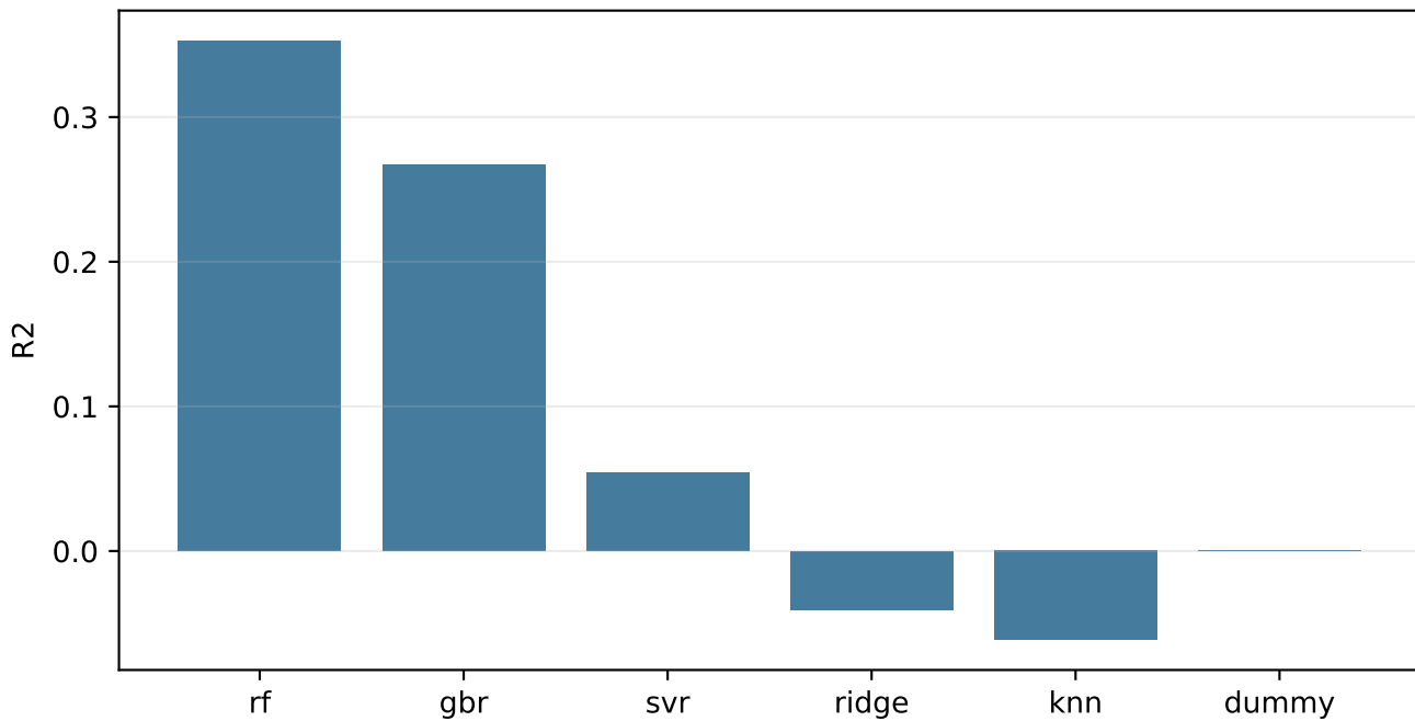
Figure 17. Classical regression validation R^2 comparison
