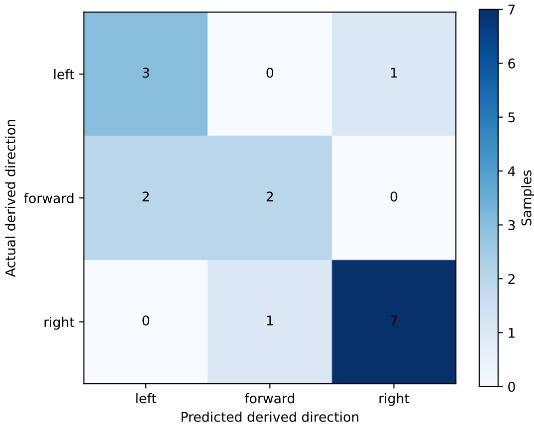
Figure 20. Directional classification confusion matrix
