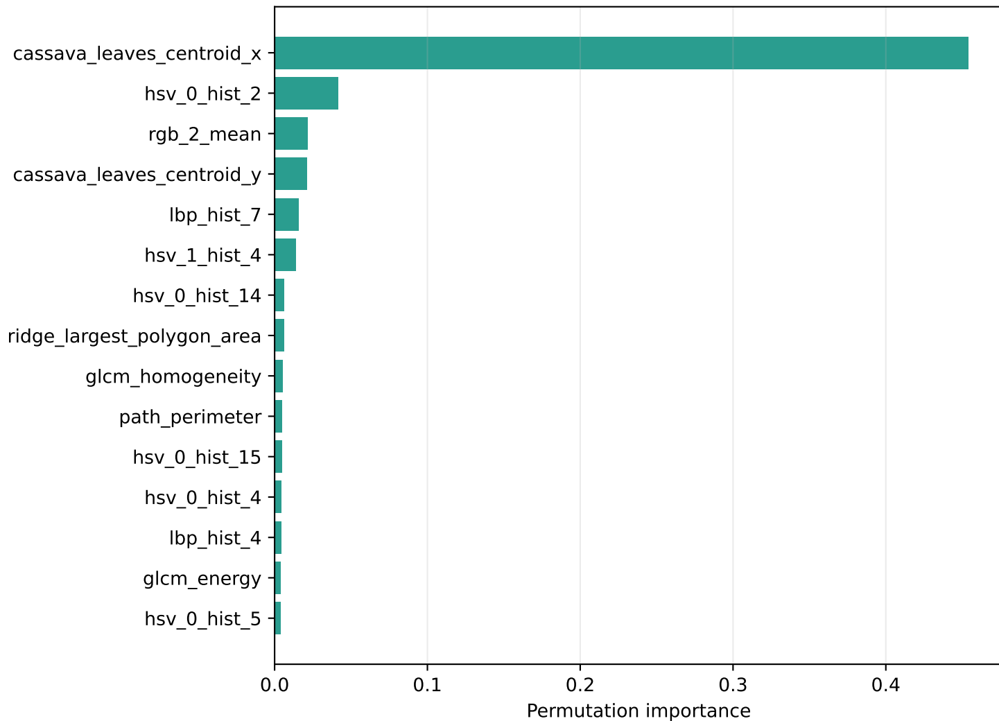
Figure 21. RF permutation feature importance
