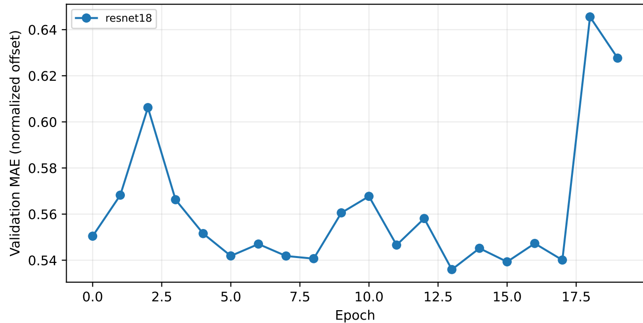
Figure 30. resnet18 validation MAE across epochs
