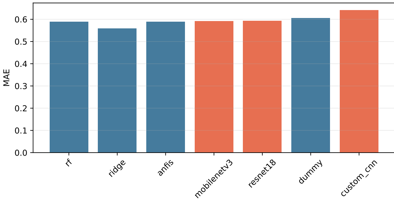
Figure 35. Overall test MAE comparison
