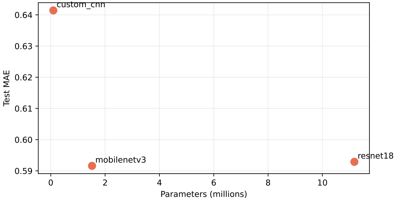
Figure 38. Deep-model size versus prediction error
