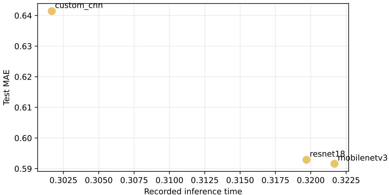
Figure 39. Deep-model latency versus prediction error
