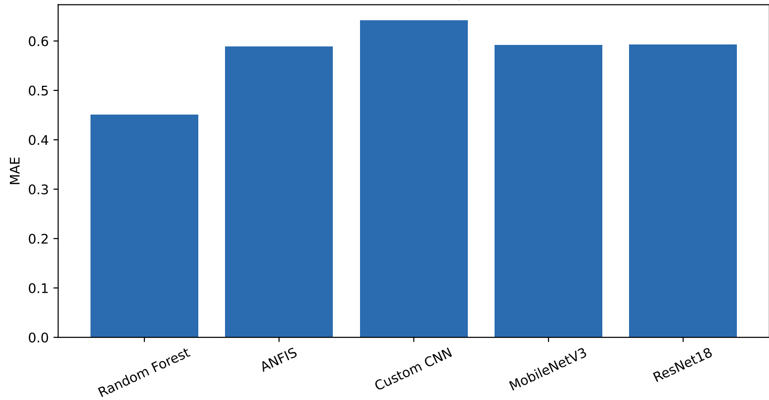
Verified test MAE by model
