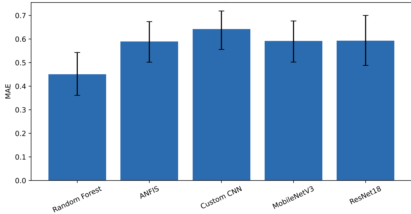
MAE with 95% bootstrap confidence intervals
