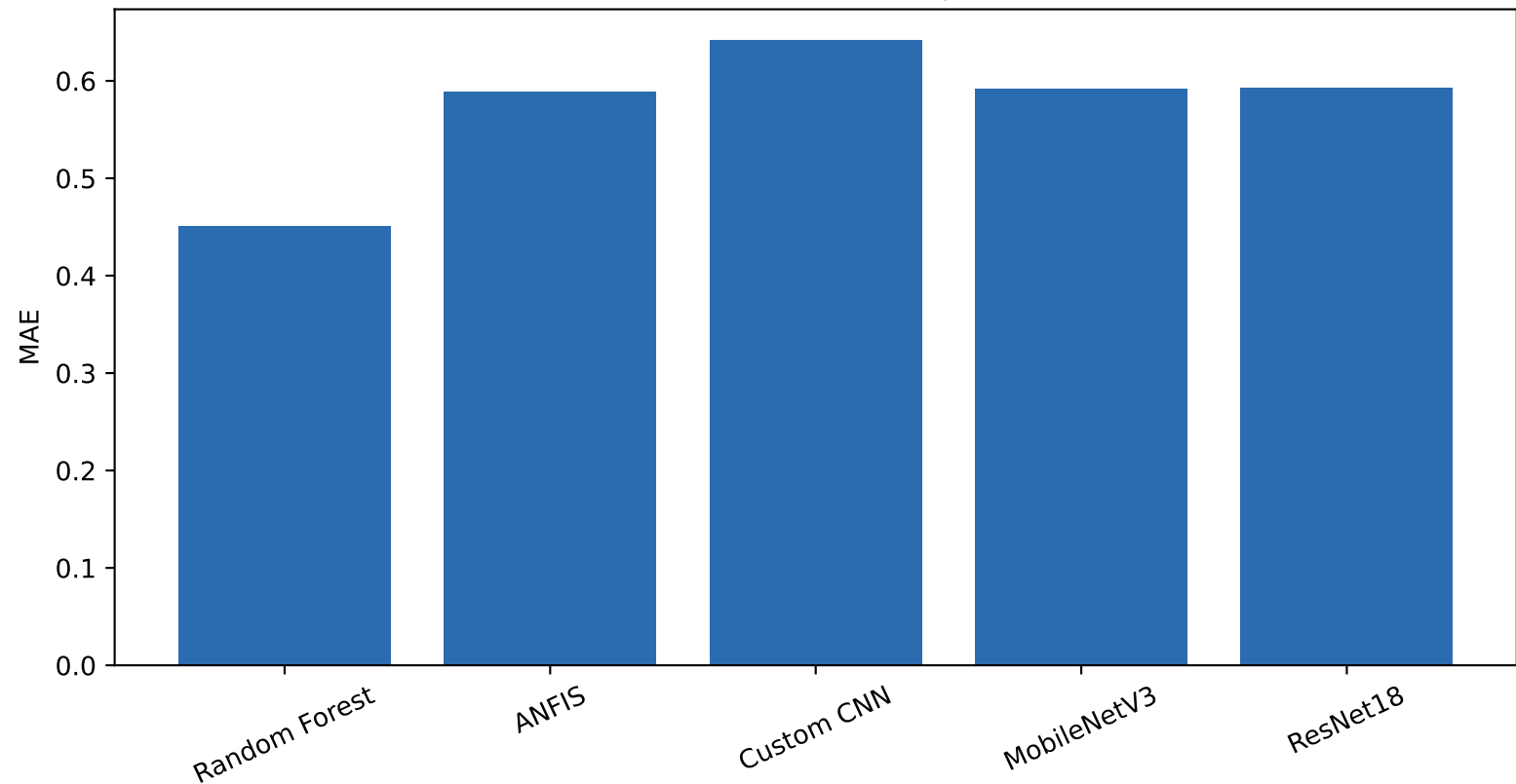
Common-test MAE comparison
