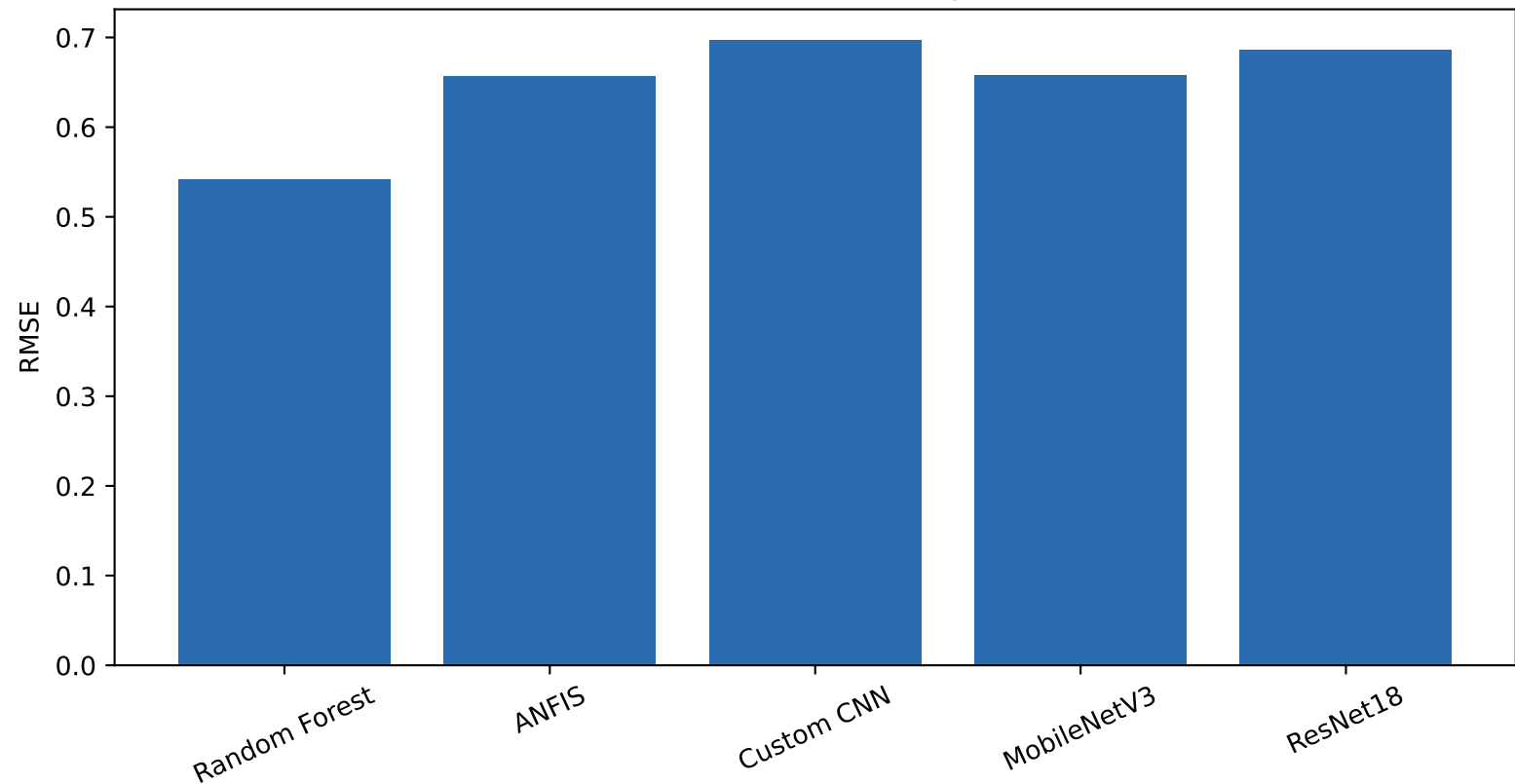
Common-test RMSE comparison
