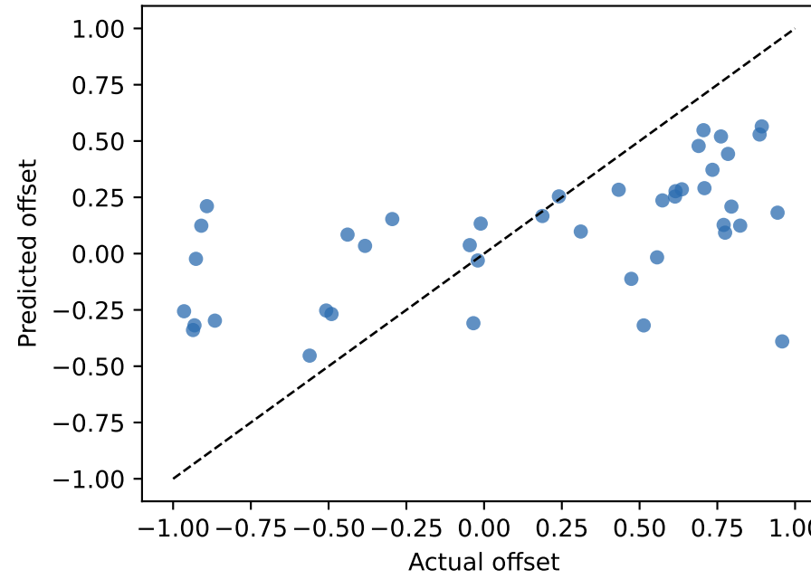
Random Forest
