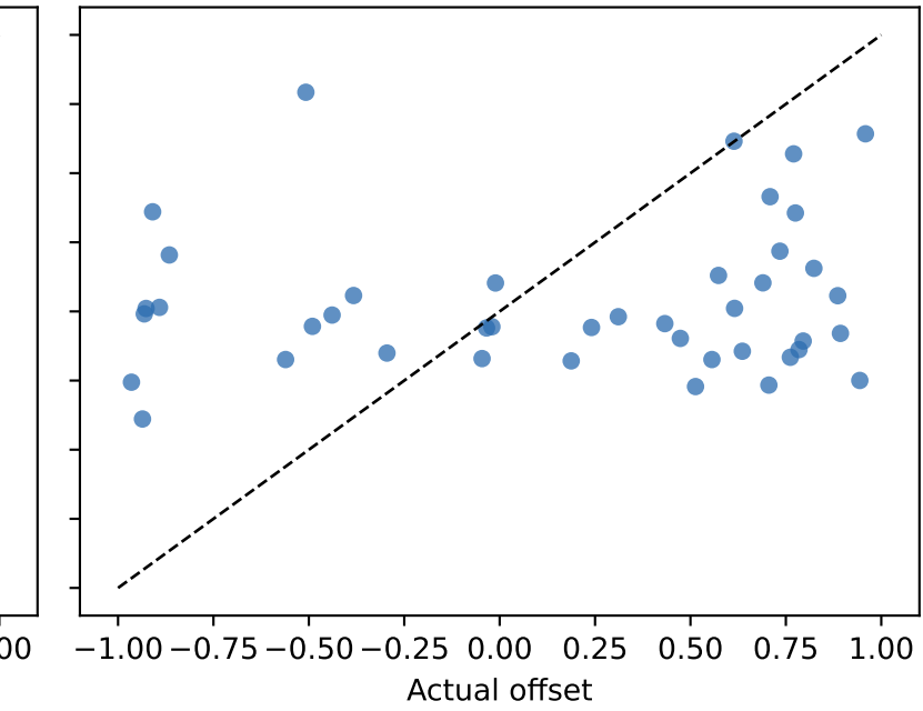
ResNet18
