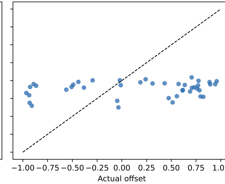
Custom CNN
