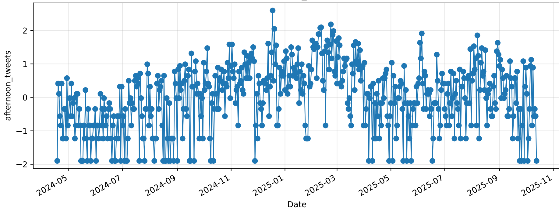
afternoon_tweets
