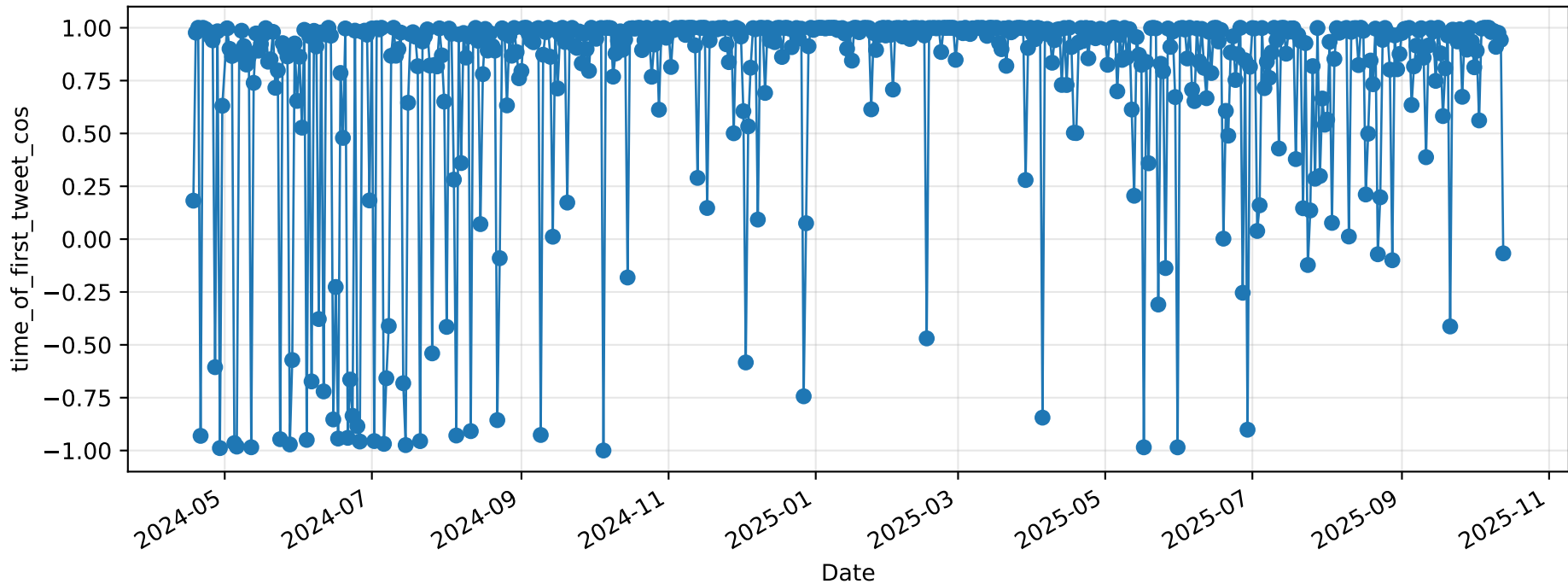
time_of_first_tweet_cos
