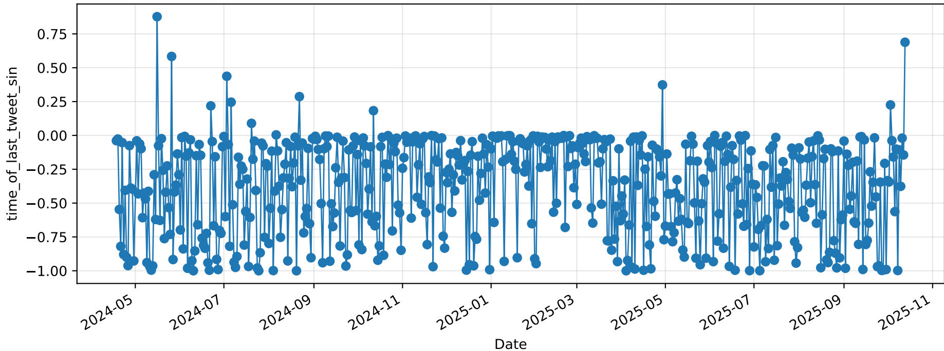
time_of_last_tweet_sin
