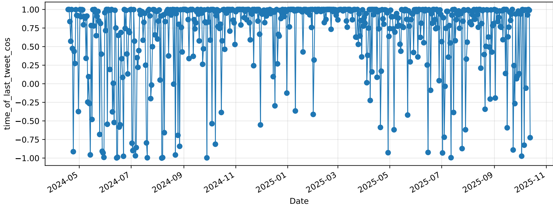
time_of_last_tweet_cos
