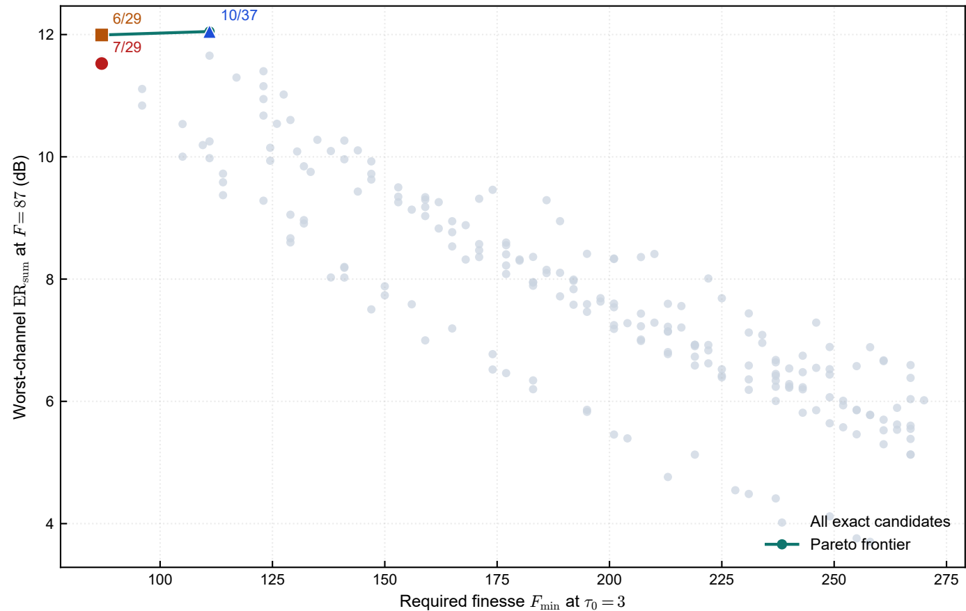
Nonuniform design trade-off: required finesse vs fixed-F worst-channel ER
