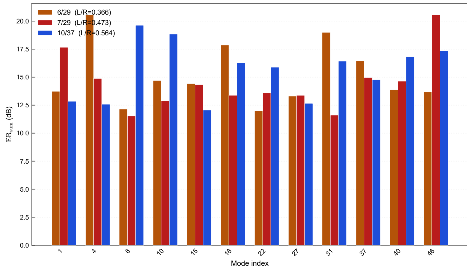
Representative candidates compared at fixed finesse F=87
