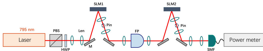
Fig. 3. Experimental setup for the nine-mode FP-cavity sorter. A tunable laser (795 nm) is beam-expanded (2.5\times) and encoded onto a reflective phase-only SLM1 via complex-amplitude holography to generate the target \text{LG}_0^l modes ( l = 0-8 ). Relay optics provide first-order selection, spatial filtering, and cavity-mode matching into a temperature-stabilized plane-concave FP cavity. The schematic shows the common input path and the mode-resolved projection arm. For mode-resolved measurements with an equal-weight superposition input, the transmitted field is projected by SLM2, relayed to a single-mode fiber, and recorded by a power meter. For spectral characterization, the cavity transmission is recorded by a photodetector at the transmission port.
