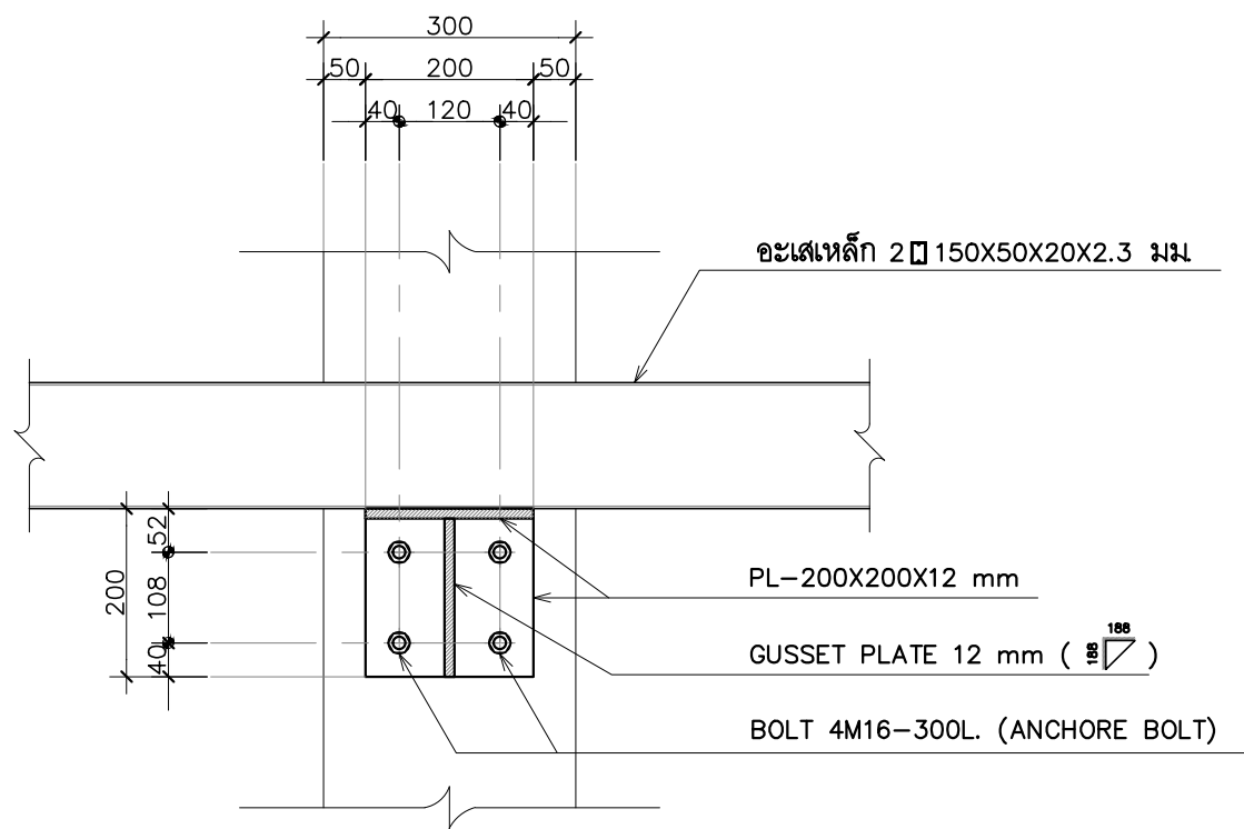
PLAN "J1"
