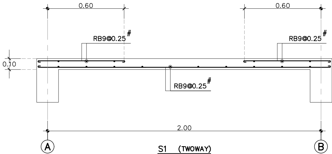
SECTION S1-S1 SCALE 1: 20
