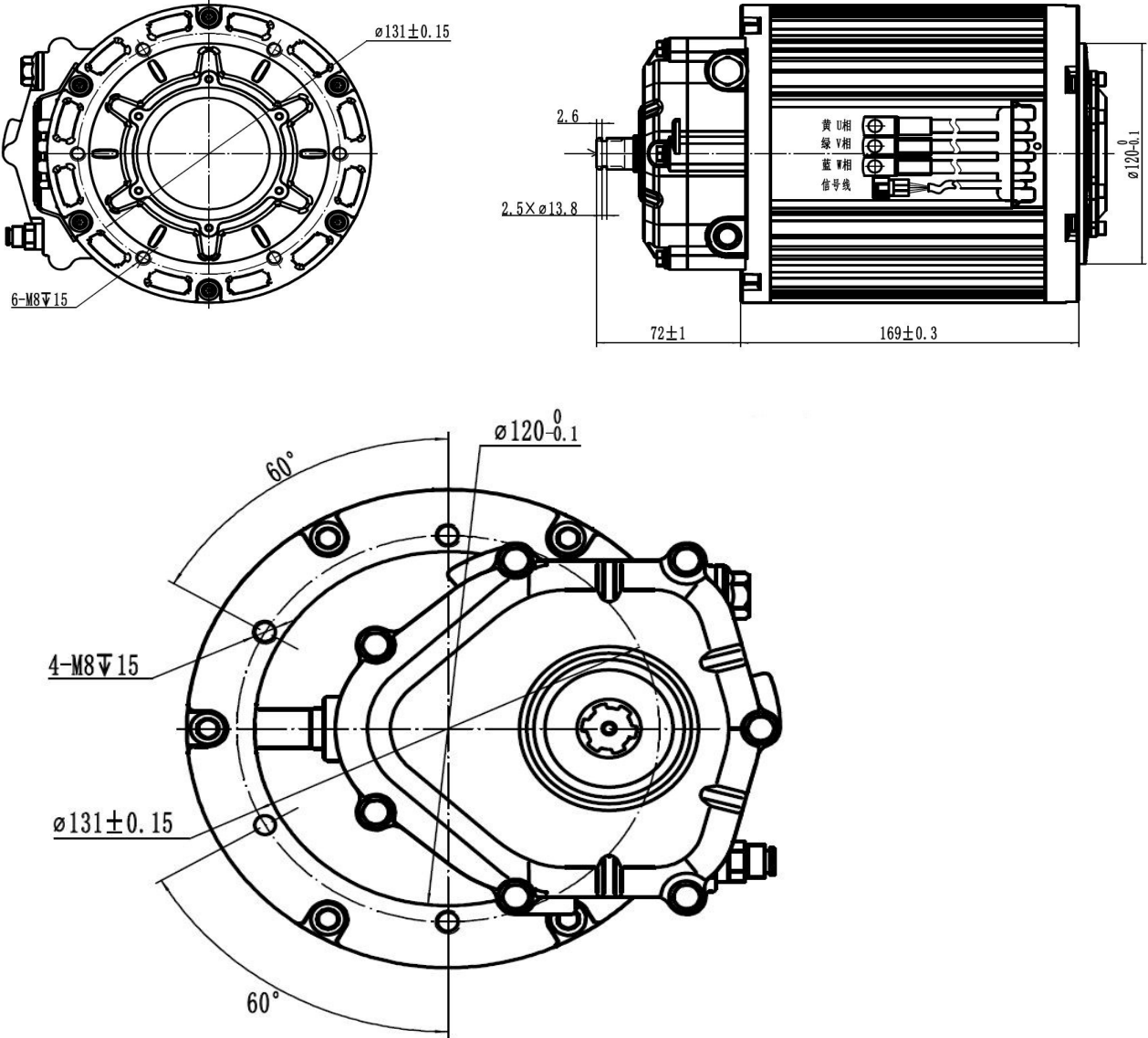
Drawing of 4000W V3 Mid Drive Motor
