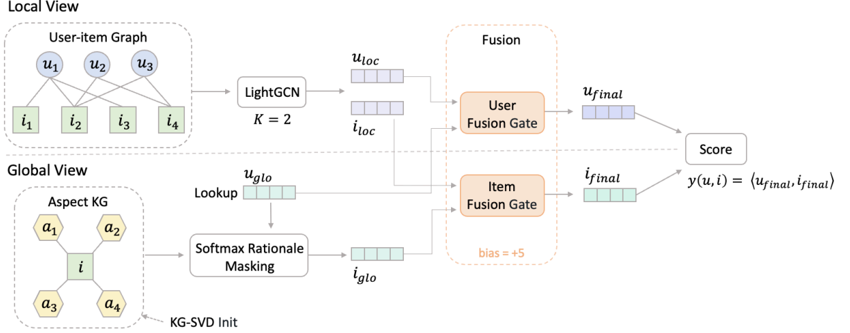
Figure 1: RA-GARK architecture.
