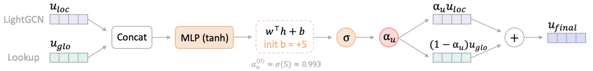
Figure 3: Local-biased fusion gate for combining local and global views.
