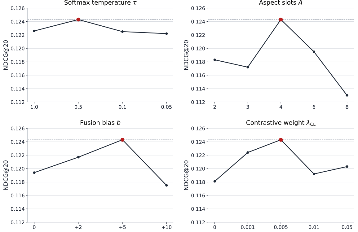
Figure 4: Sensitivity of RA-GARK to the four main hyperparameters under NDCG@20.
