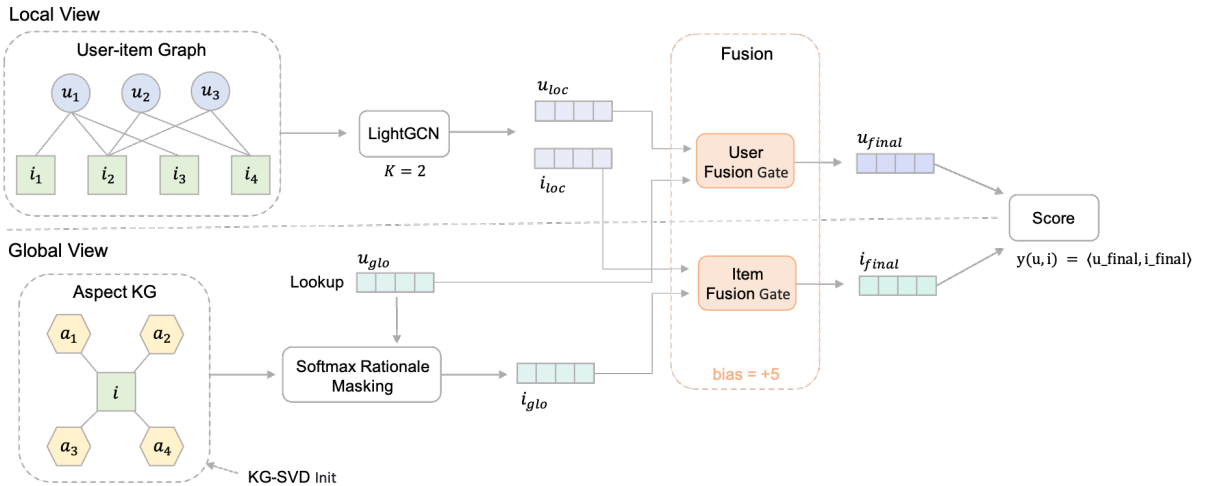
Figure 1: RA-GARK architecture.
