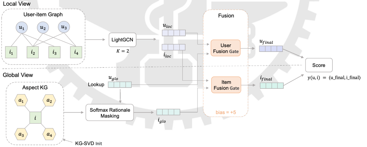
Figure 1: RA-GARK architecture.
