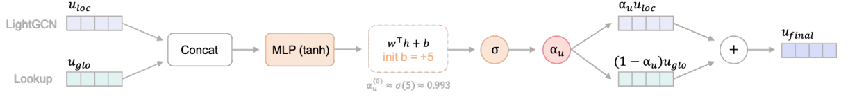
Figure 3: Local-biased fusion gate.
