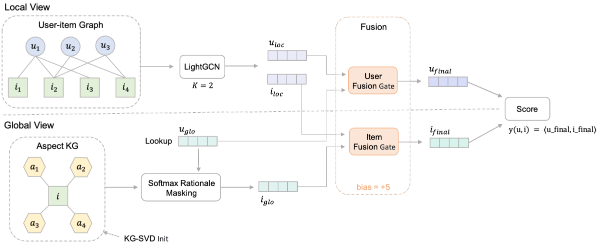
Figure 1: RA-GARK architecture.
