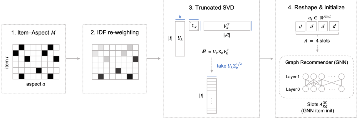
Figure 2: KG-SVD initialization of item aspect slots.
