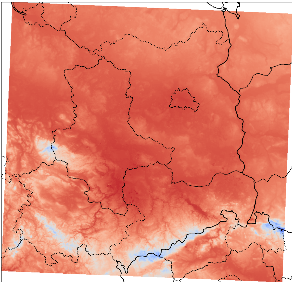
Mean temperature through 1961-1992
