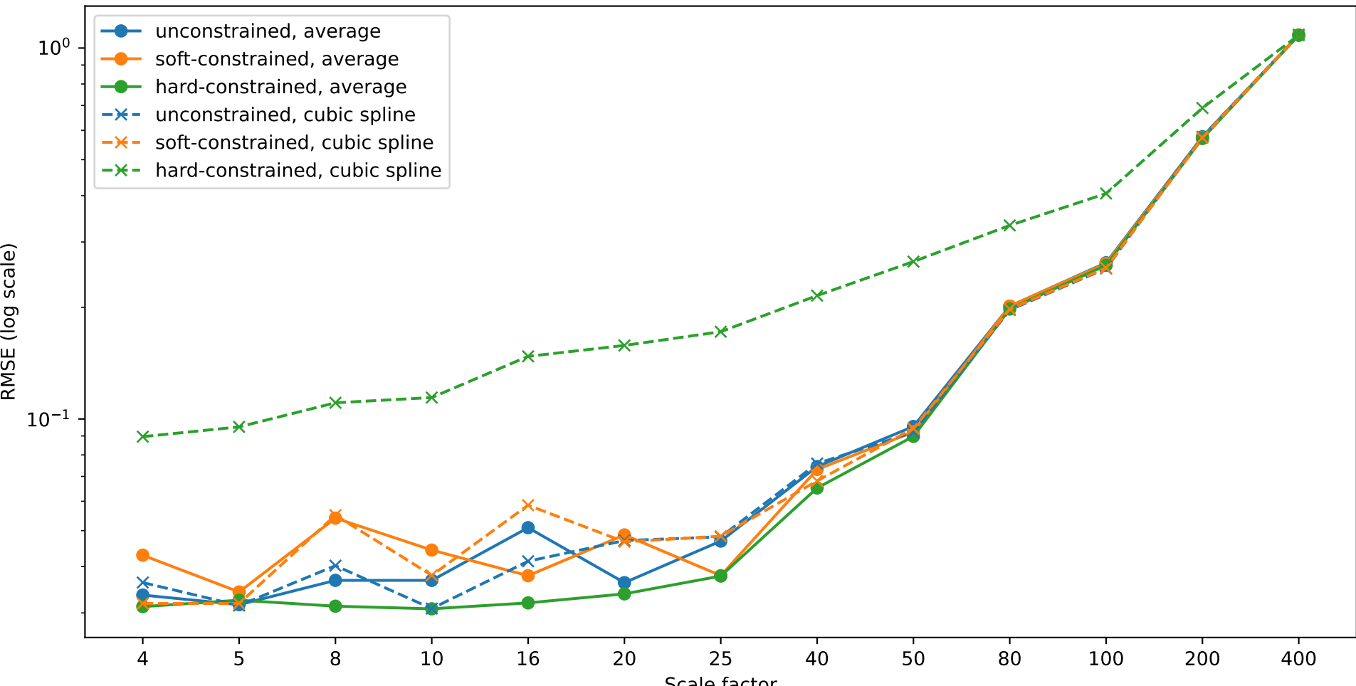
RMSEs of constraining and resampling combinations
