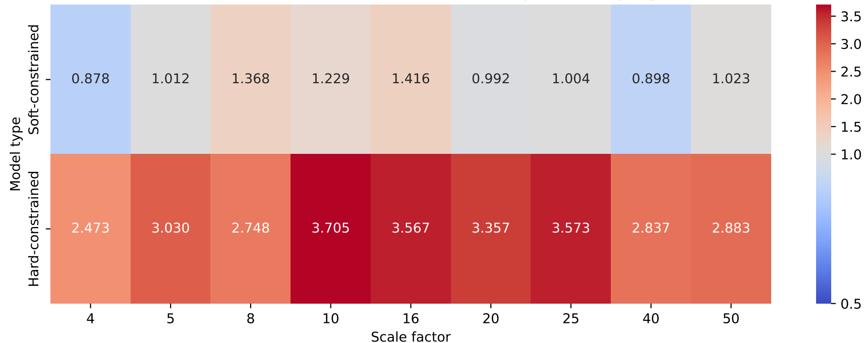
RMSE ratio relative to the baseline for the cubic spline resampling runs
