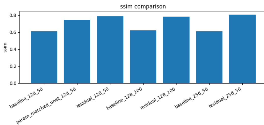
SSIM comparison across experiments.
