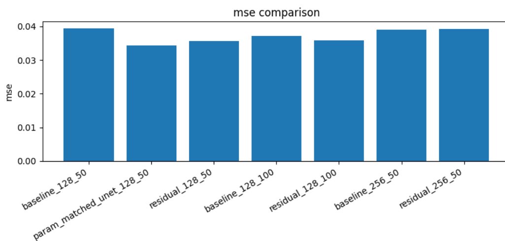
MSE comparison showing the capacity-control effect.
