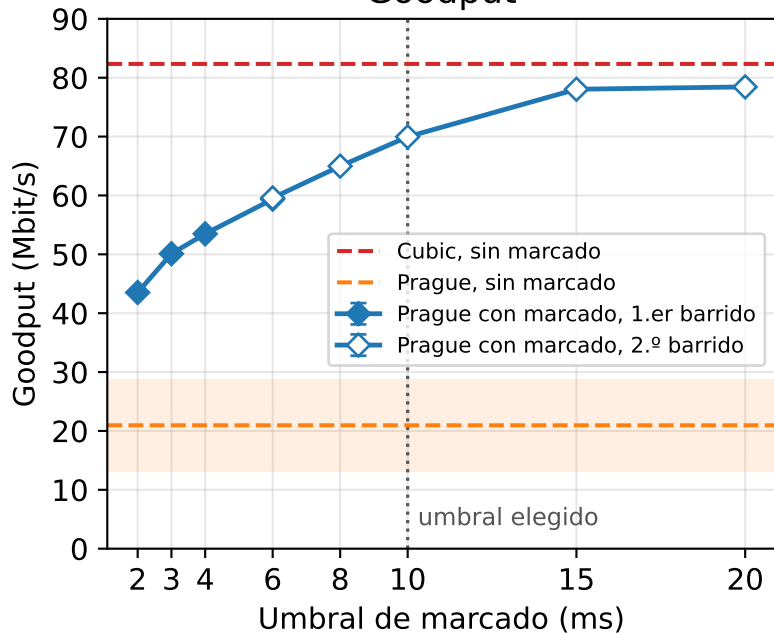
Goodput
