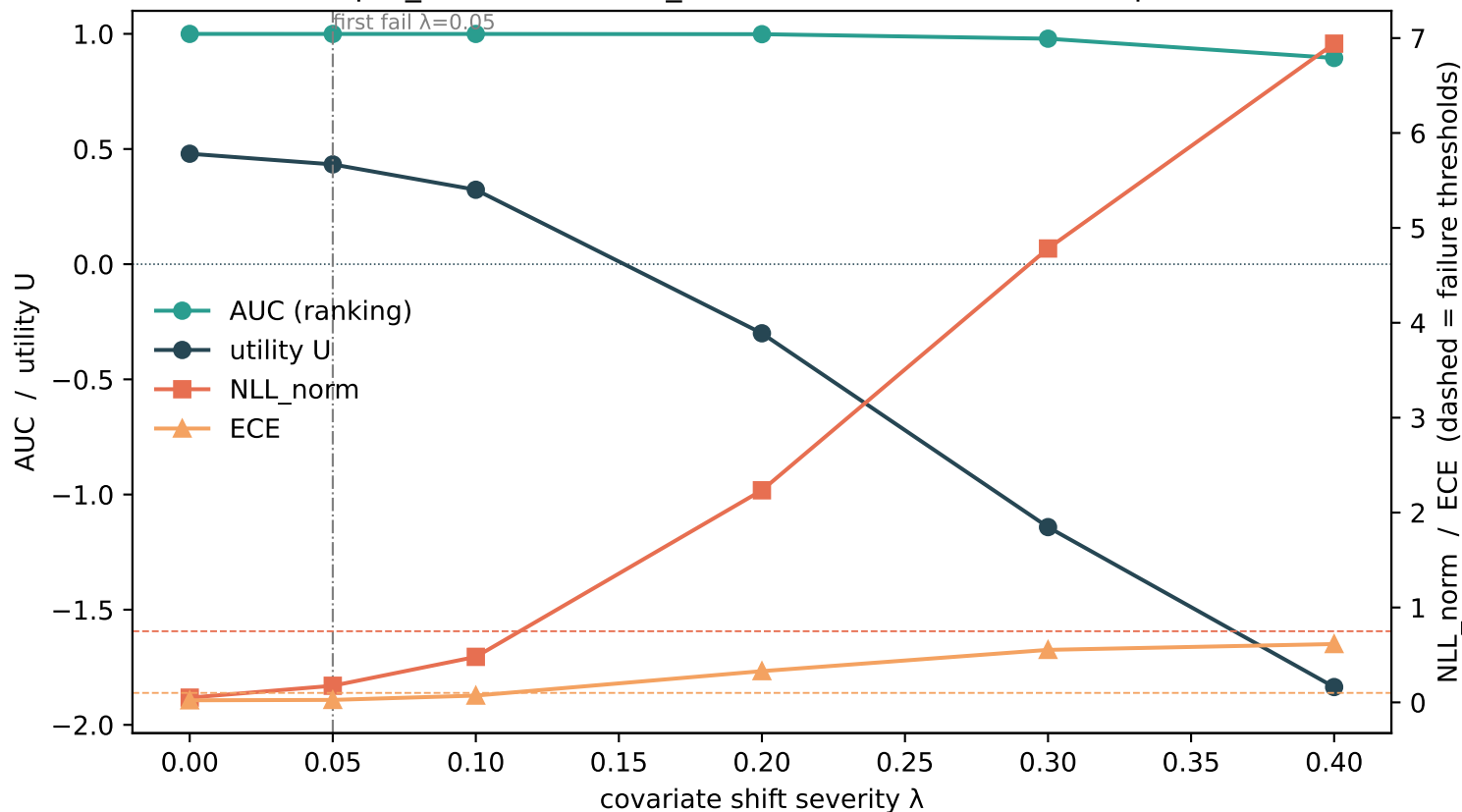
Covariate shift breaks calibration, not discrimination (tabpfn_client on breast_cancer: AUC flat, NLL/ECE explode)
