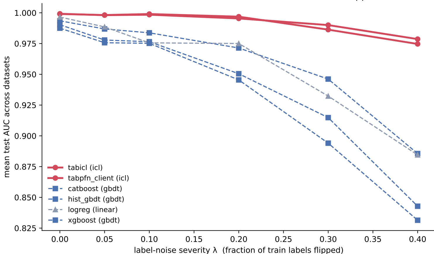
Label noise: in-context models resist, GBDTs memorise the flipped labels
