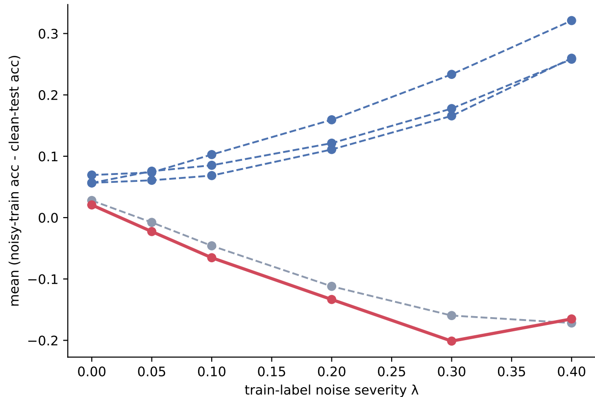
Train-label noise: ICL models retain clean-test ranking while GBDT baselines degrade faster
