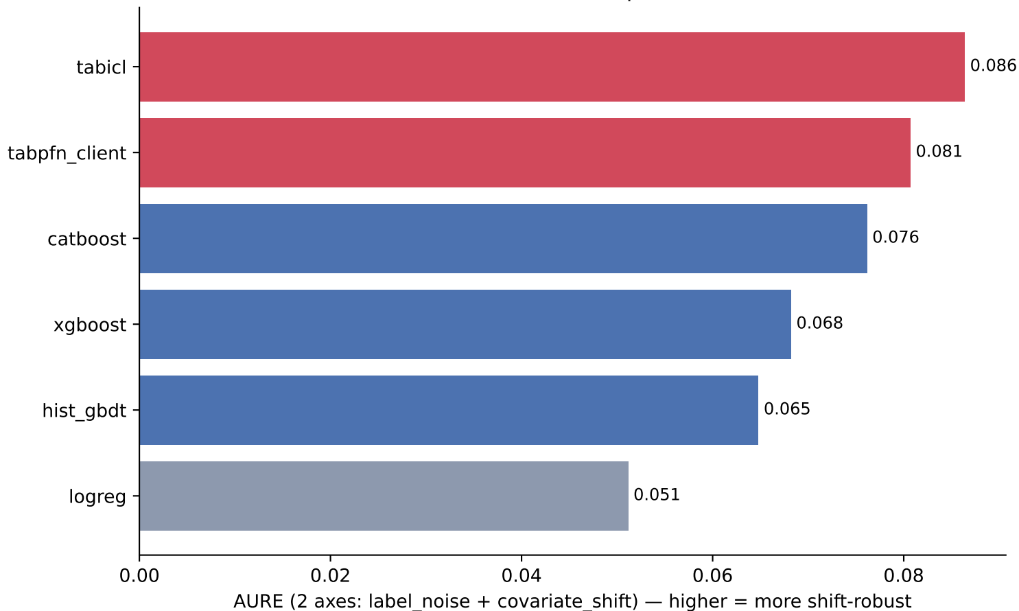
External validation — AURE per model (2-axis)
