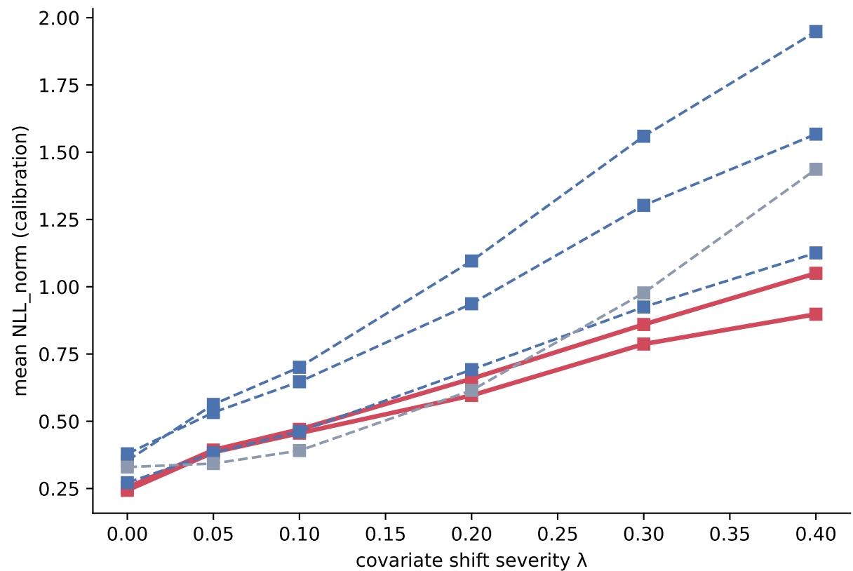
External: covariate shift — discrimination holds while calibration degrades
