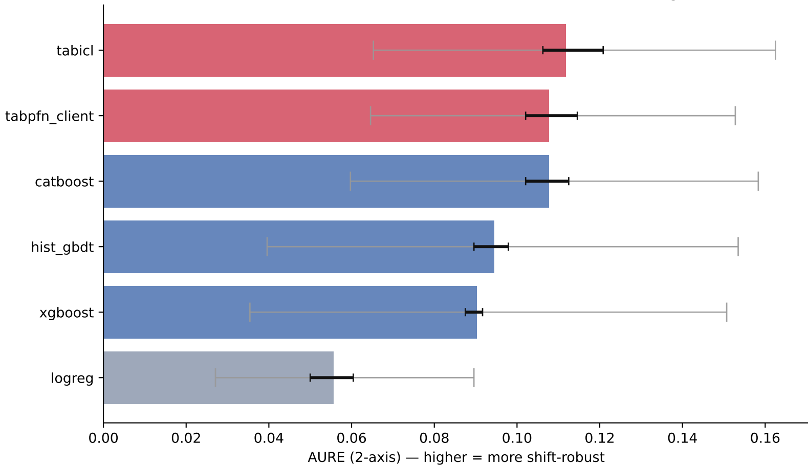
Stratified external (12 datasets, 3 seeds): AURE — dark=seed CI, light=dataset CI
