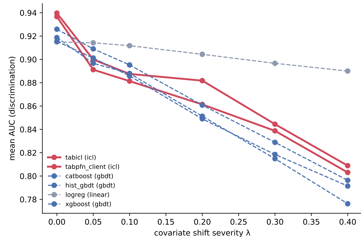
Stratified external: covariate shift — calibration degrades faster than discrimination
