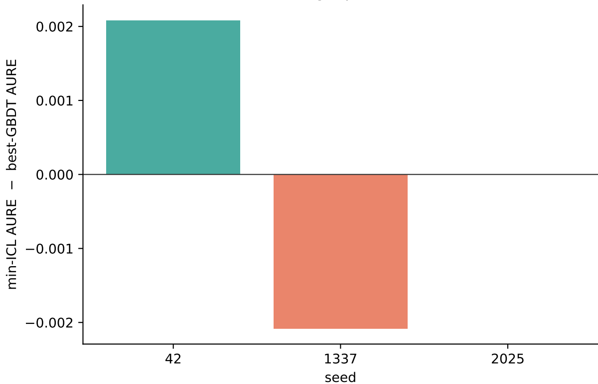
ICL vs best-GBDT margin per seed (mean +0.000)
