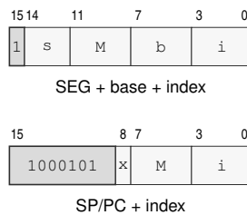
Figure 7-3. EXT0 Two-Byte Indexed Descriptor Byte Layouts
