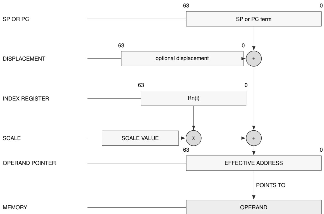
Schema — EXT2 SP/PC indexed
