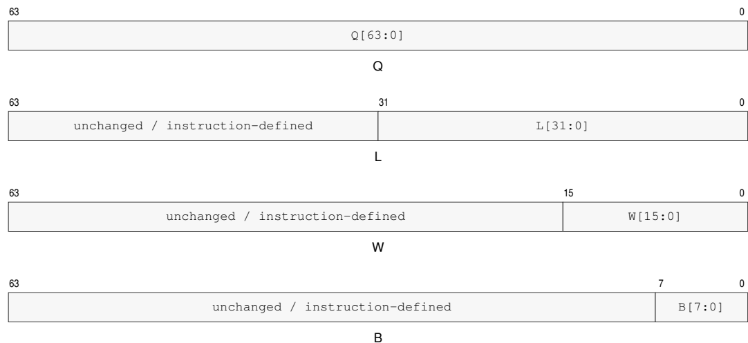
Figure 5-1. Rn Register Operand Subfields
