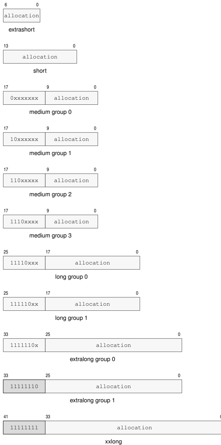
Figure 6-2. Opcode-space Allocation Namespaces
