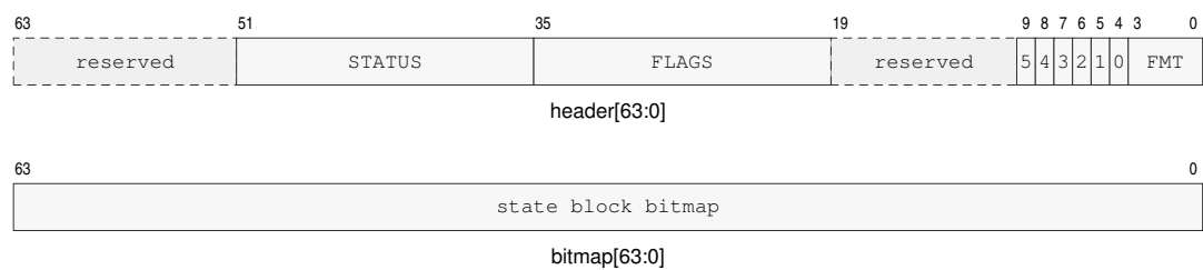
Figure 16-1. SAVE/RESTORE Base Header
