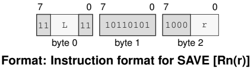
Format: Instruction format for SAVE [Rn(r)]
