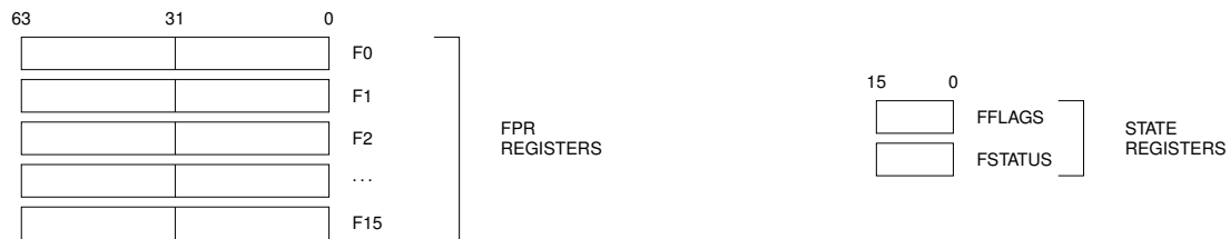
Figure 3-4. FP Register Model
