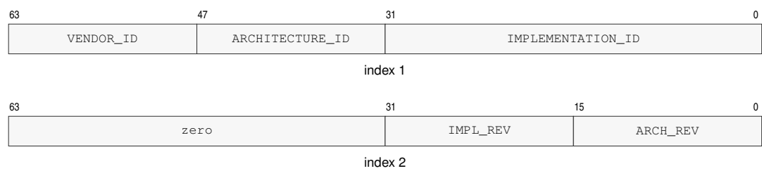
Figure 15-3. CPUID Base Identity Result Formats
